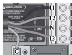
3-phases with single neutral
