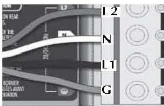
For 240 V (4 wires)
