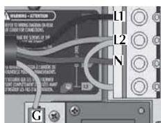
2-phases with single neutral
