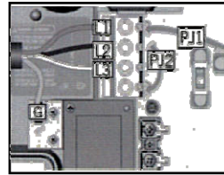
3-Phases Delta
