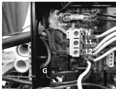
240V (4 wires)
